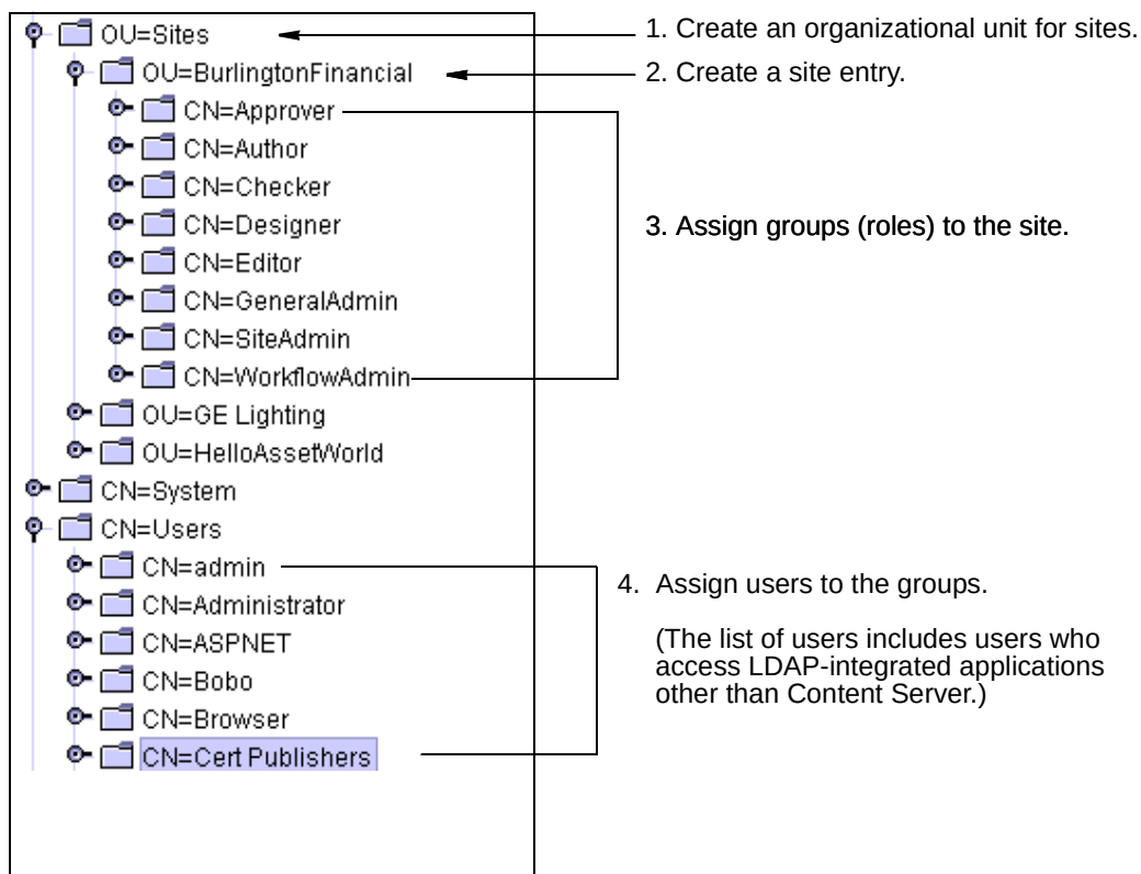
Figure 1: LDAP Hierarchies
