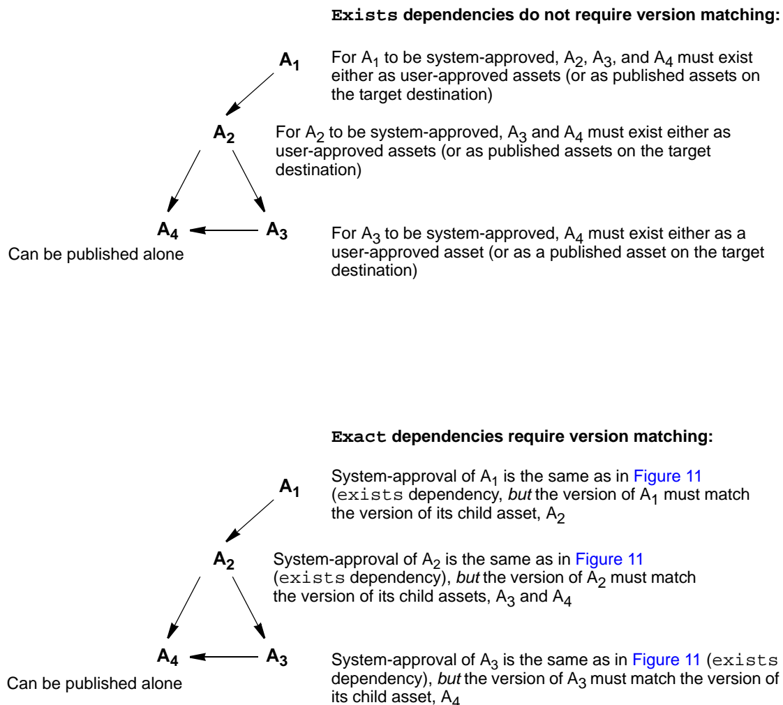
Figure 11: Exists/Exact Dependencies
