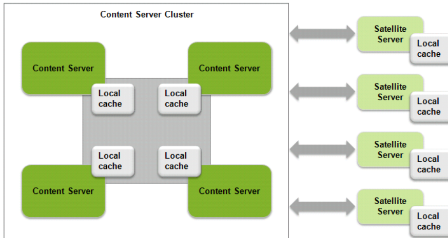
Figure 18: Local Caches
