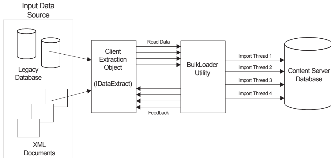
Figure 8: Client-specific implementation of BulkLoader
