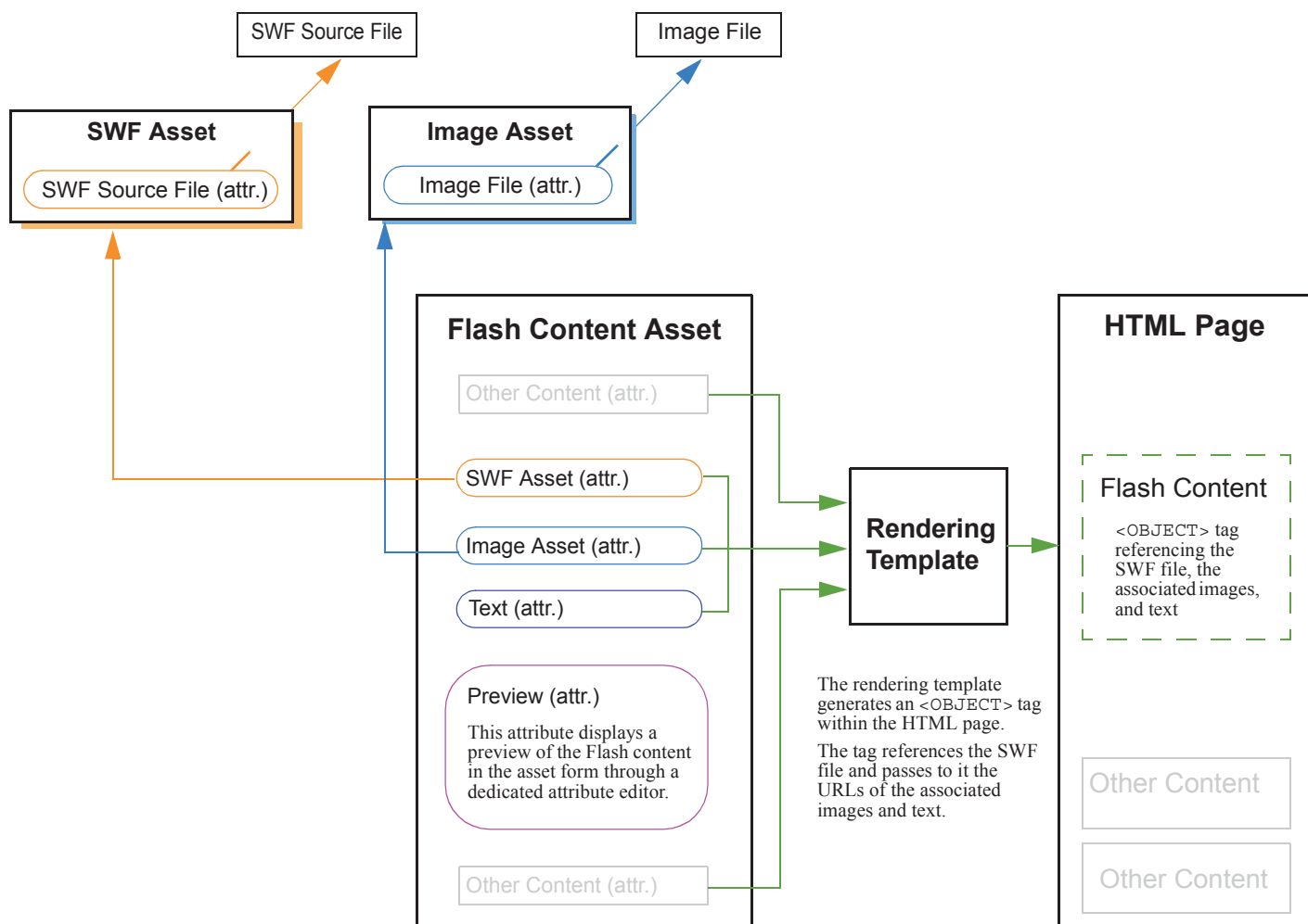
Figure 14: Flash Management Model
