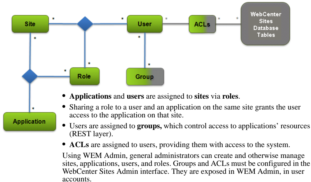
Figure 2: Authorization Model
